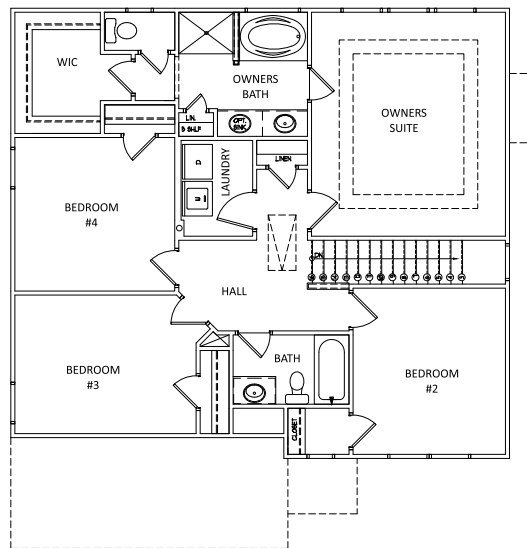
SECOND FLOOR
