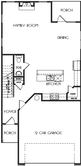
ASHTON 1ST FLOOR PLAN
