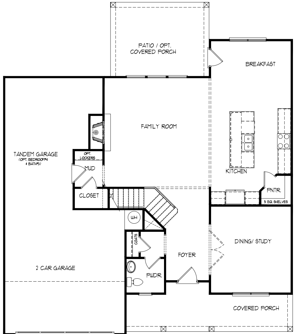
MAIN FLOOR
